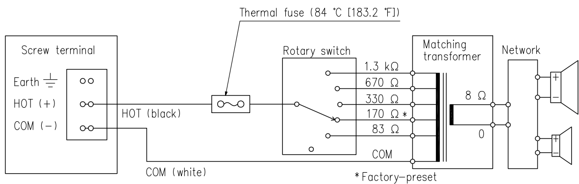
Wiring Diagram
